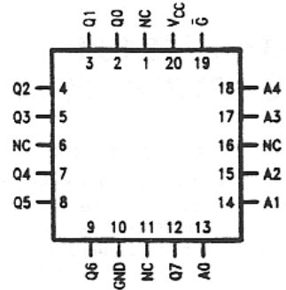
Plastic Leaded Chip Carrier (PLCC)
